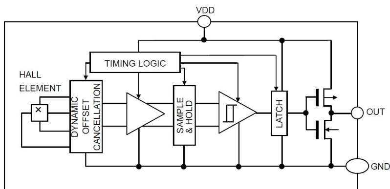
Figure 3, Block Diagram of AS1918
