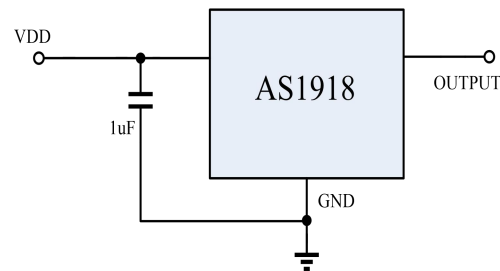
Figure 1, Typical Application Circuit of AS1918
