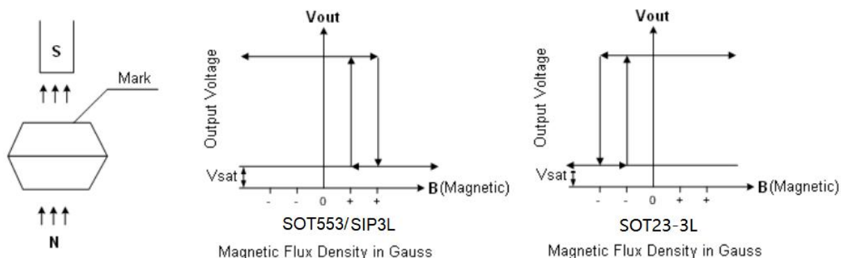
Fig 4, Magnetic Operation Characteristic of AS1918
